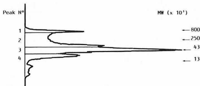
Fig. 1. Size-exclusion high-performance liquid chromatography elution curve of sodium dodecyl sulfate-phosphate buffer extract of durum wheat, cultivar Kidur.
