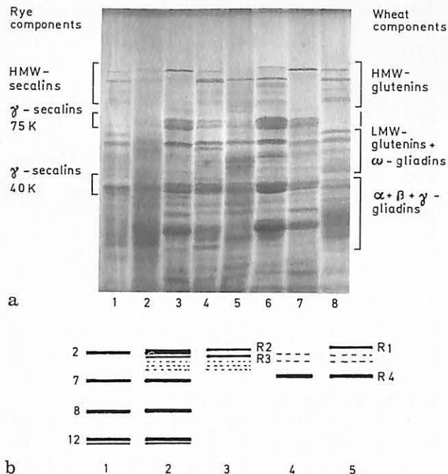
Fig. 1. a SDS-PAGE patterns of the total seed proteins contained in the following samples: 1 "FEC 28" wheat; 2 rye line no. 571; 3 rye line no. 51; 4 "Clercal" triticale; 5 triticale 4x line no. 532 S 10; 6 triticale 8x line no. T 206; 7 rye line no. 51; 8 "Etoile de Choisy" wheat. b Schemes of the high-molecular-weight secalin or glutenin patterns of the following samples: 1 "FEC 28" and "Etoile de Choisy" wheats; 2 triticale 8x line no. T 206; 3 rye line no. 51; 4 triticale 4x line no. 532 S 10; 5 rye line no. 571
