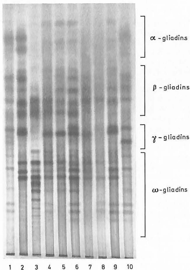
Fig. 3. PAGE patterns of gliadins contained in the following samples: 1 "Etoile de Choisy" wheat; 2 "Clercal" triticale; 3 rye line no. 51; 4 triticale T 249; 5 triticale T 254; 6 triticale T 68; 7 triticale T 206; 8 triticale T 217; 9 triticale T 231; 10 "Etoile de Choisy" wheat
