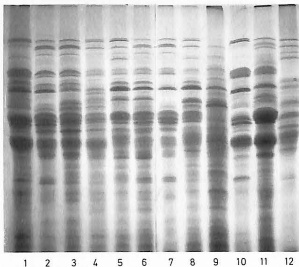
Fig. 4. SDS-PAGE patterns of the total seed proteins contained in the following lines of the T 8x \times T 4x progeny: 1 rye line no. 51; 2 triticale T 29; 3 triticale T 30; 4 triticale T 52; 5 triticale T 76; 6 triticale T 77; 7 triticale T 216; 8 triticale T 217; 9 triticale 4x line no. 532 S 10; 10 rye line no. 51; 11 rye line no. 571; 12 "Etoile de Choisy" wheat
