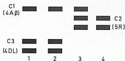
Fig. 2. Scheme of the \beta -amylase zymograms of the following samples: 1 "FEC 28" wheat; 2 triticale 8x T 206; 3 triticale 4x line no. 532 S 10; 4 rye line no. 51. The chromosome control of the C_1 , C_2 , and C_3 components is indicated
